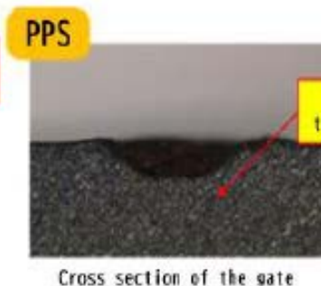
Cross section of the gate
